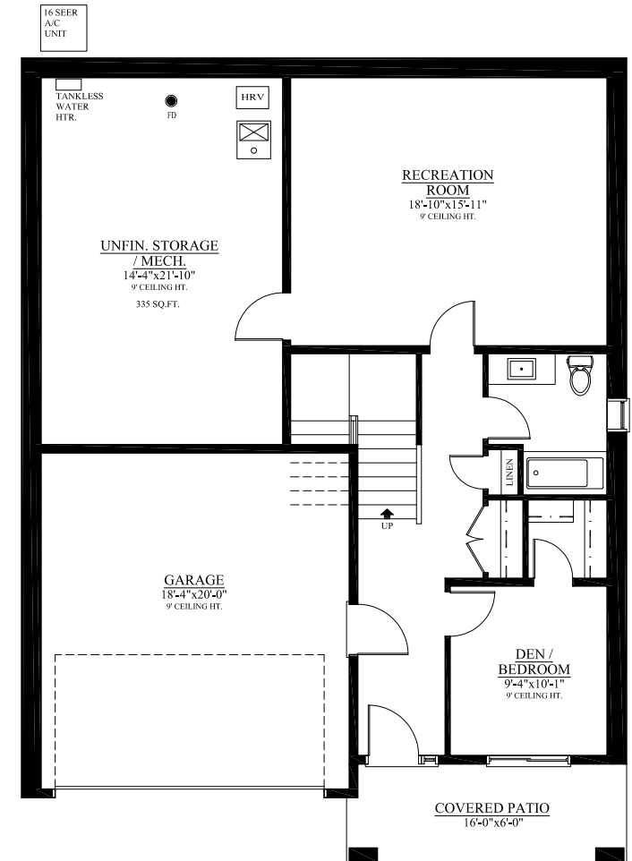
LOWER FLOOR PLAN 679 SQ. FT.
